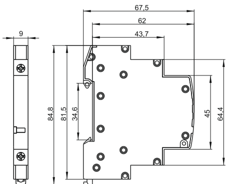
a) 1 LED
