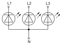
b) 3 LED
