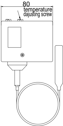
Dimension (unit: mm)
