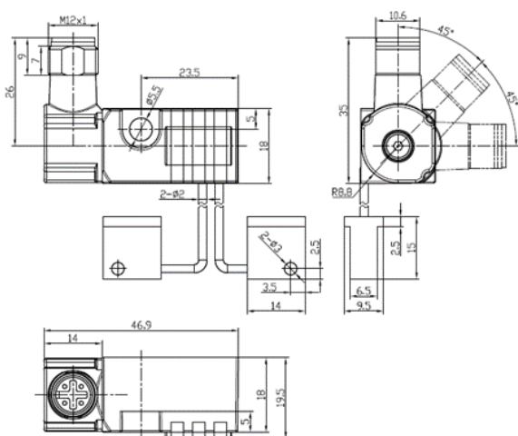
NPN NO+NO
