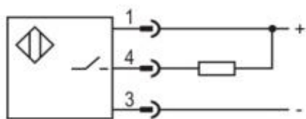
NPN NO
