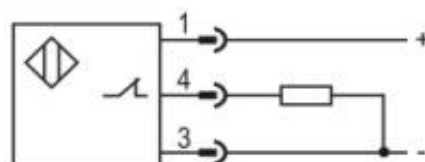
PNP NC
