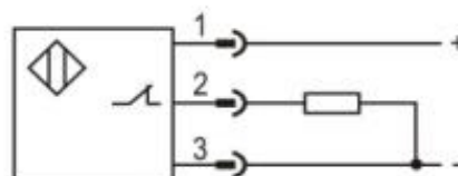
PNP NC
