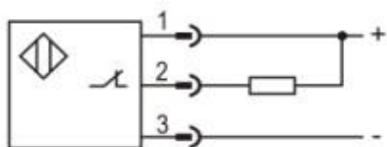
NPN NC
