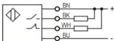
NPN NO+NC
