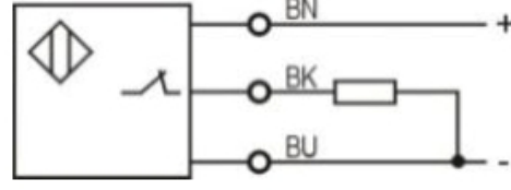
PNP NC
