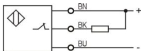
NPN NC
