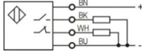
PNP NO+NC
