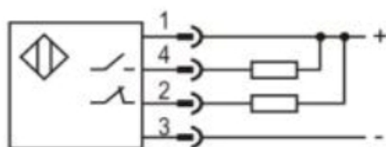
NPN NO+NC
