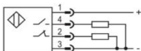
PNP NO+NC
