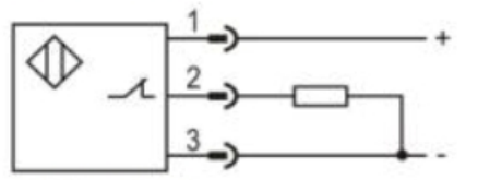
PNP NC
