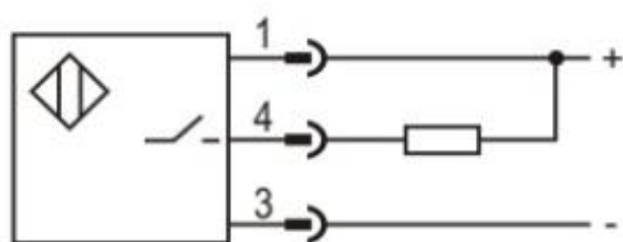
NPN NO
