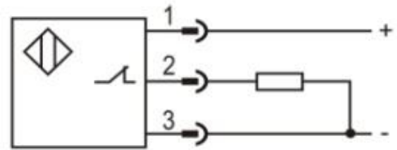
PNP NC
