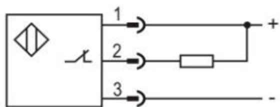
NPN NC
