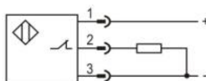
PNP NC
