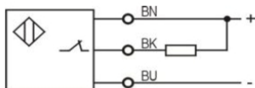
NPN NC
