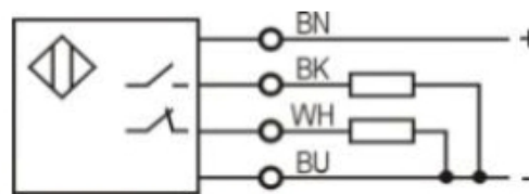
PNP NO+NC
