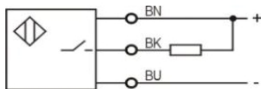
NPN NO
