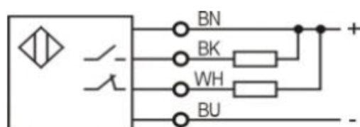
NPN NO+NC
