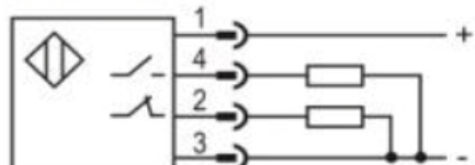
PNP NO+NC
