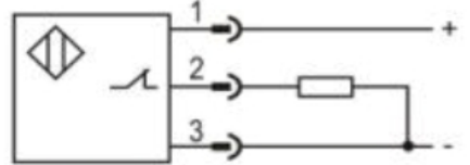
PNP NC
