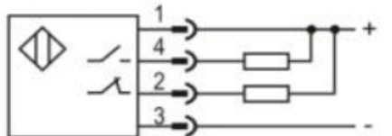
NPN NO+NC
