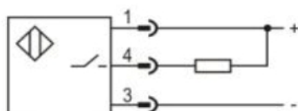
NPN NO
