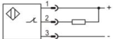
NPN NC
