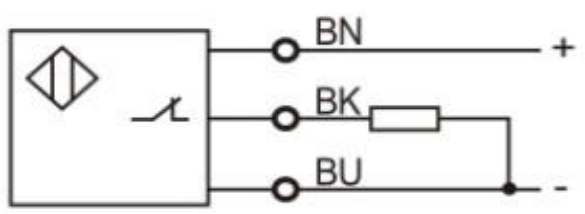
PNP NC
