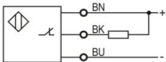
NPN NC
