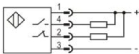
NPN NO+NC
