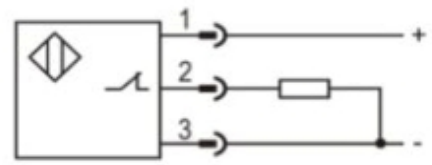
PNP NC
