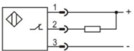
NPN NC
