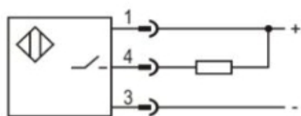
NPN NO
