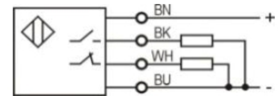
PNP NO+NC
