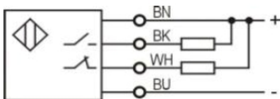
NPN NO+NC
