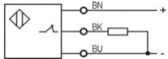
PNP NC
