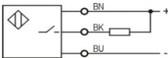
NPN NO
