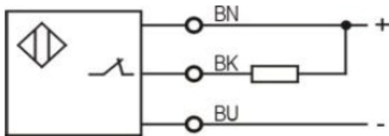
NPN NC
