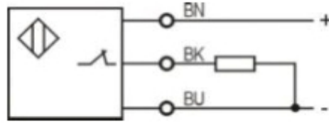
PNP NC
