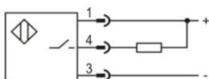
NPN NO
