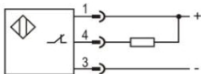
NPN NC
