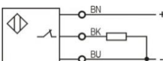
PNP NC
