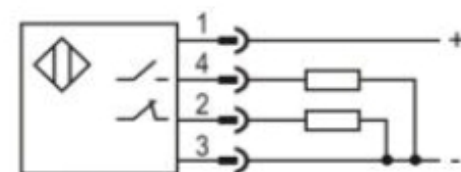
PNP NO+NC
