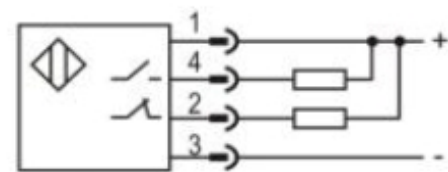
NPN NO+NC
