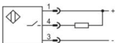
NPN NO
