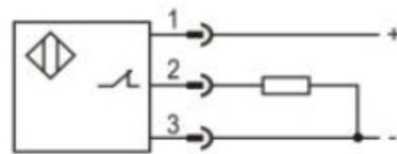
PNP NC
