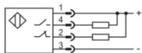
NPN NO+NC
