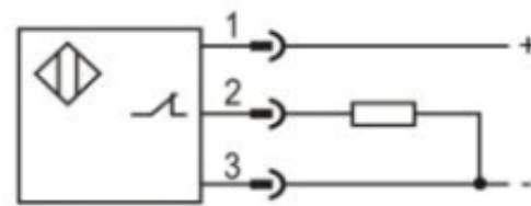
PNP NC
