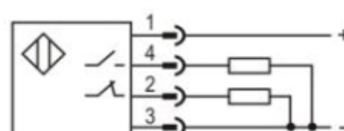
PNP NO+NC
