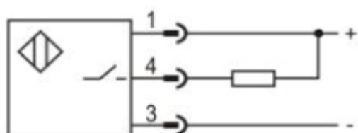
NPN NO
