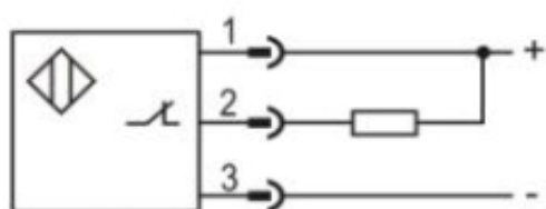
NPN NC
