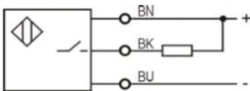
NPN NO
