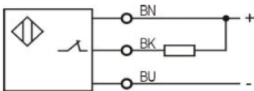
NPN NC
