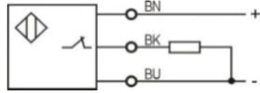
PNP NC
