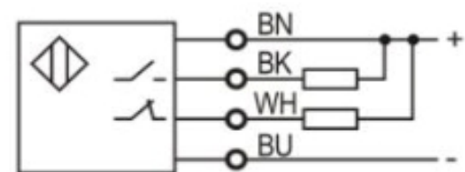
NPN NO+NC
