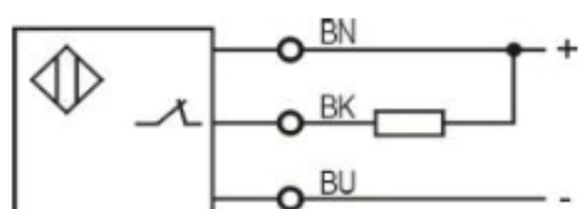
NPN NC
