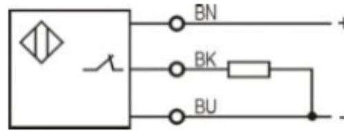
PNP NC
