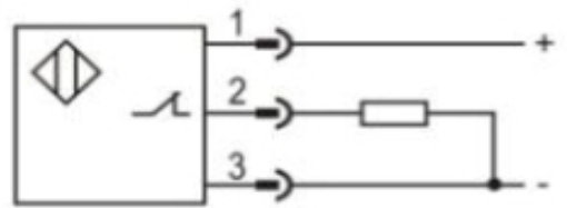
PNP NC
