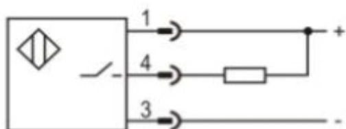
NPN NO
