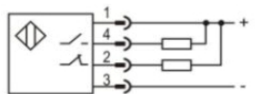
NPN NO+NC
