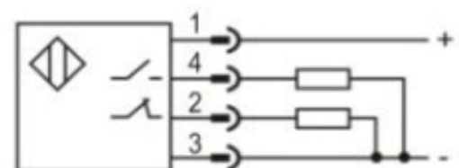
PNP NO+NC
