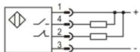
NPN NO+NC
