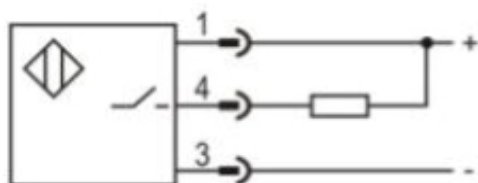
NPN NO
