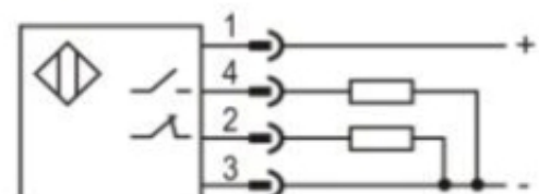
PNP NO+NC
