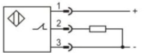
PNP NC
