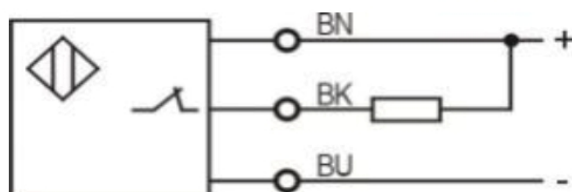
NPN NC
