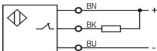
NPN NC
