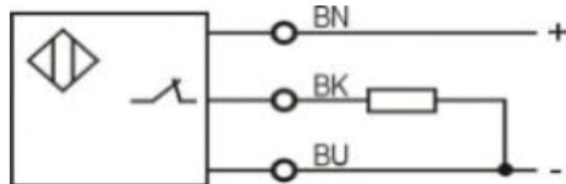
PNP NC
