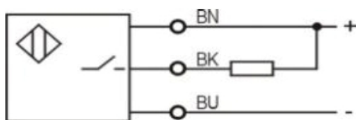
NPN NO
