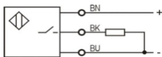
NPN NC
