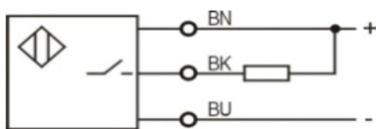
NPN NO
